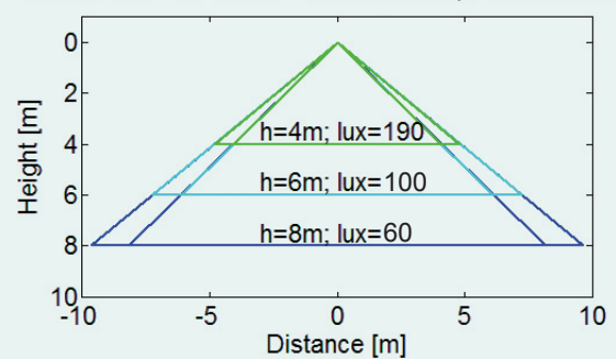
Athos 400 + GI-CX01 + 72x Cree Xte, Emission cone
