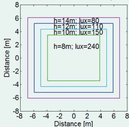
Athos 400 + GI-ST01 + 72x Cree Xte, Ground spot
