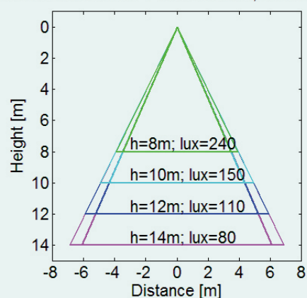
Athos 400 + GI-ST01 + 72x Cree Xte, Emission cone
