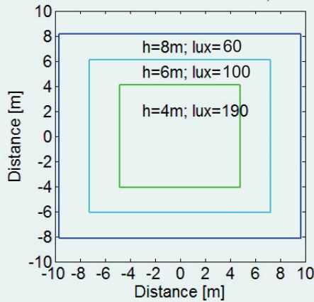
Athos 400 + GI-CX01 + 72x Cree Xte, Ground spot
